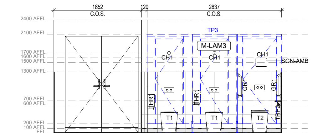
5 Area 51 - Amenities - Male - Elevation 1 1:50
