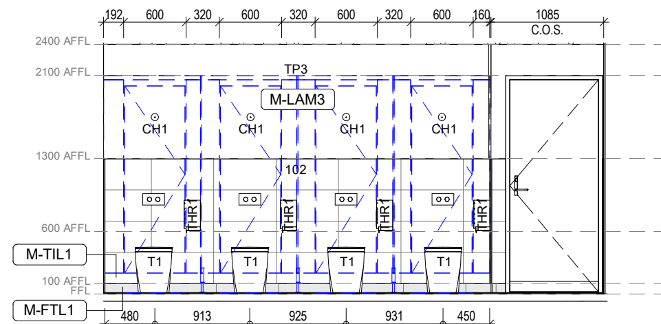
3 Area 51 - Amenities - Female - Elevation 3 1:50
