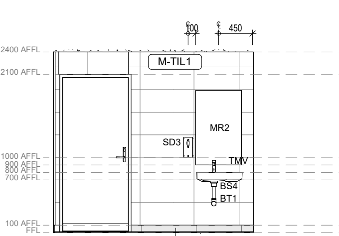
10 Area 51 - PWD Elevation 2 1:50
