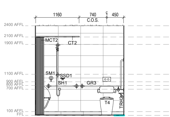
12 Area 51 - PWD Elevation 4 1:50
