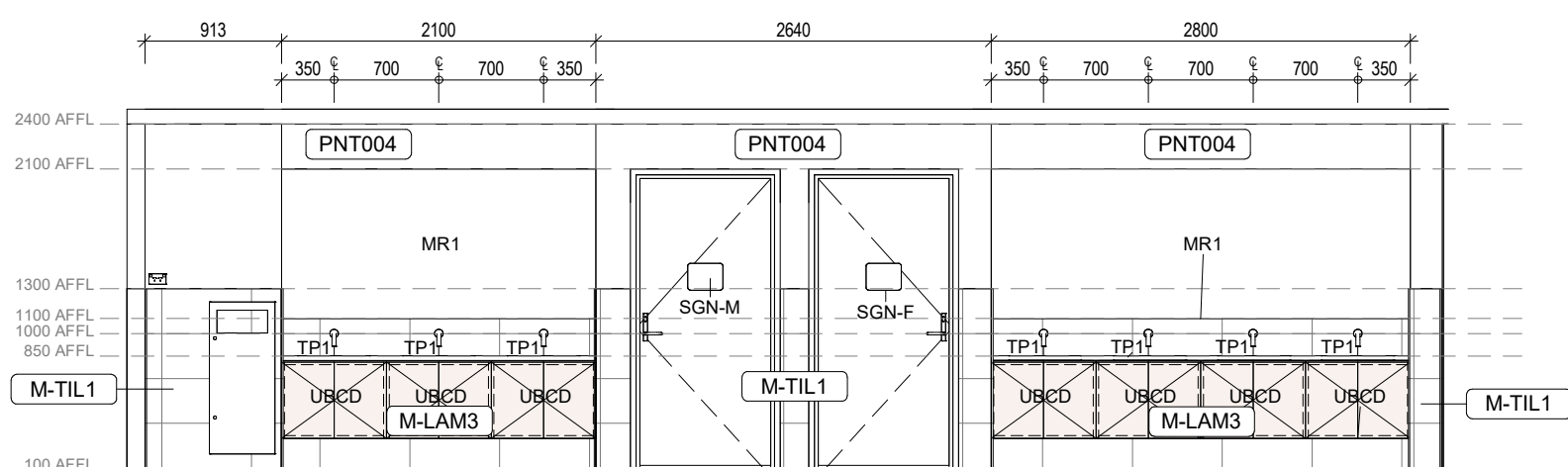
14 Area 51 - Corridor & Handwash Area Elevation 2 1:50
