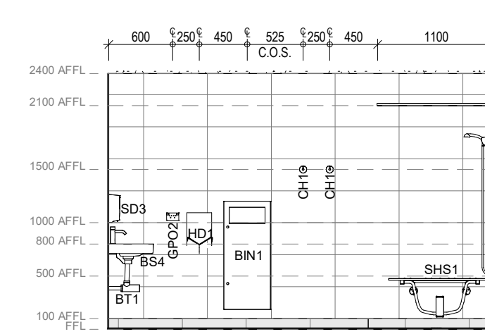
11 Area 51 - PWD Elevation 3 1:50
