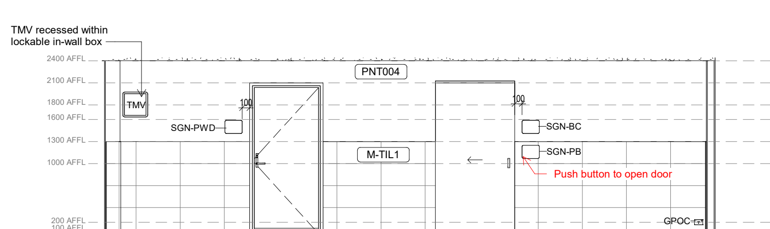
16 Area 51 - Corridor & Handwash Area Elevation 4 1:50
