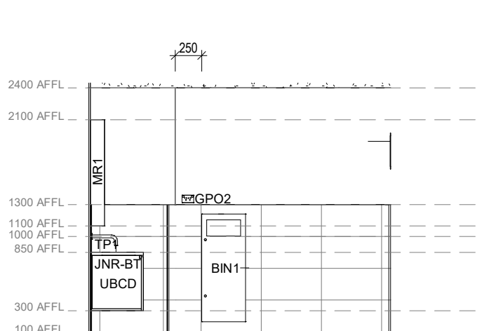
15 Area 51 - Corridor & Handwash Area Elevation 3 1:50
