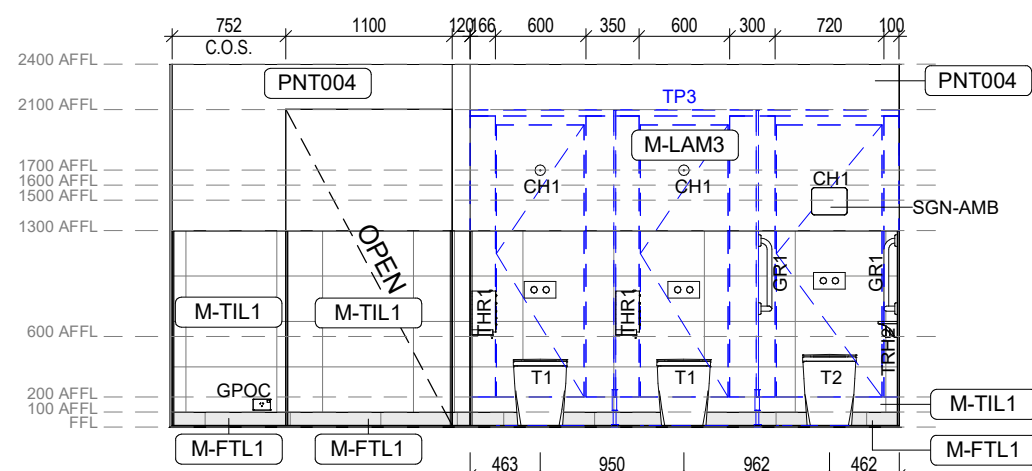
1 Area 51 - Amenities - Female - Elevation 1 1:50
