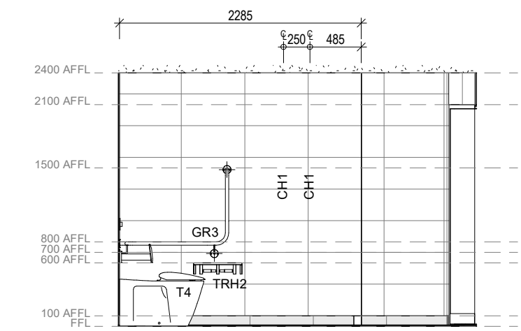
9 Area 51 - PWD Elevation 1 1:50
