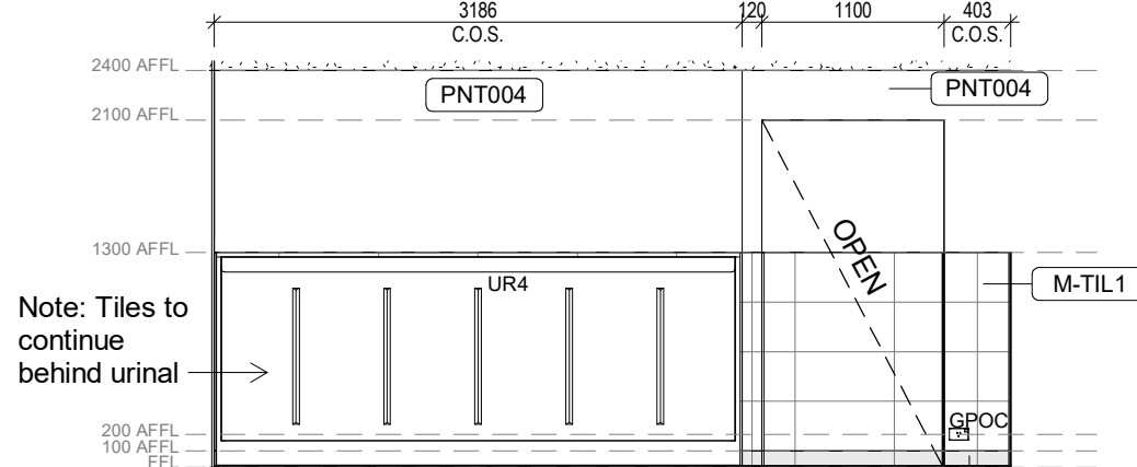
7 Area 51 - Amenities - Male - Elevation 3 1:50
