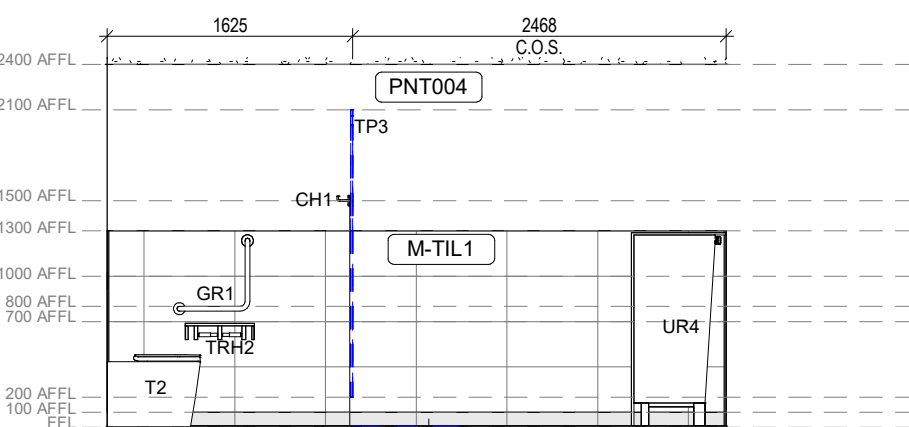
6 Area 51 - Amenities - Male - Elevation 2 1:50
