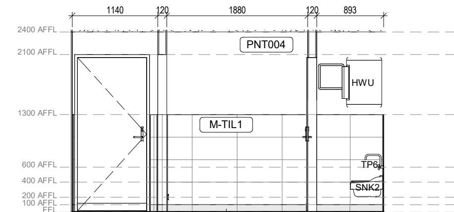
8 Area 51 - Amenities - Male - Elevation 4 1:50
