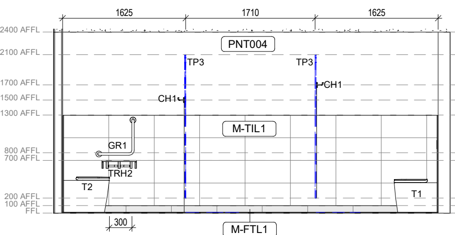
2 Area 51 - Amenities - Female - Elevation 2 1:50
