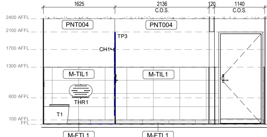
4 Area 51 - Amenities - Female - Elevation 4 1:50
