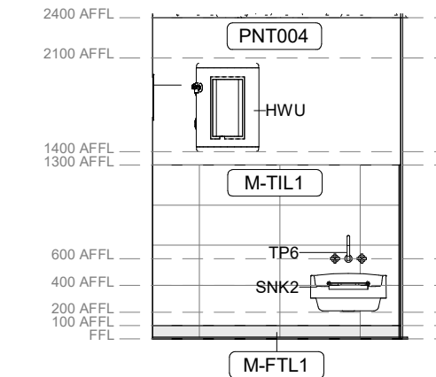
17 Area 51 - Cleaners Elevation 1 1:50
